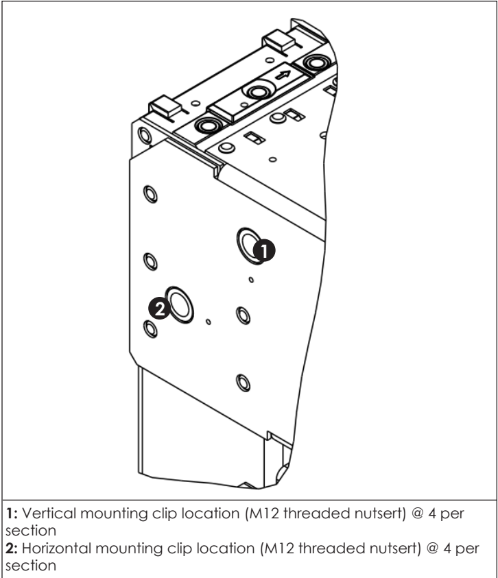
Figure 4: Mounting Clip Attachment Points
