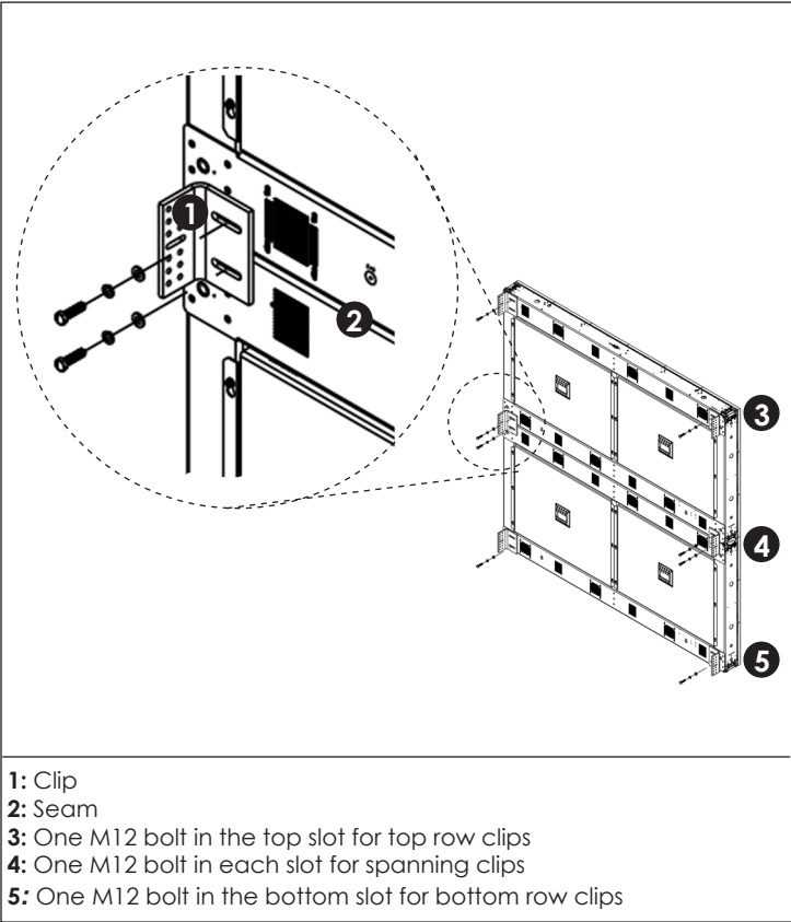
Figure 2: Display (Rear View)
