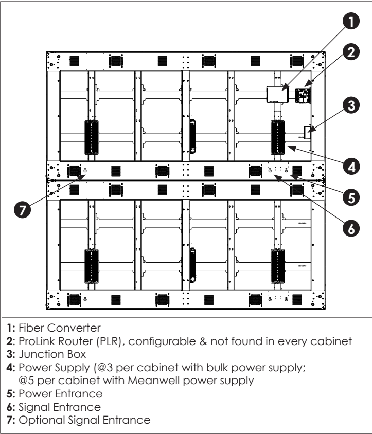
Figure 6: Component Locations (Rear View)
