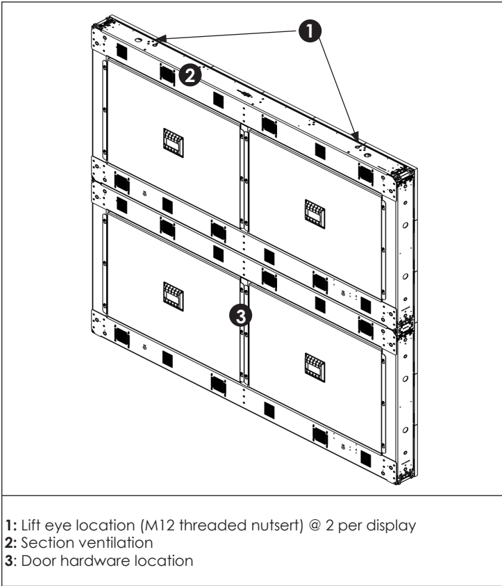
Figure 1: Display (Front View)
