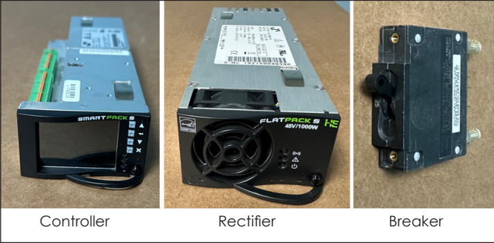
Figure 7: Eltek Components
