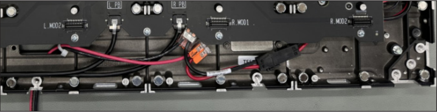
Figure 6: Wired Power Connection at Display
