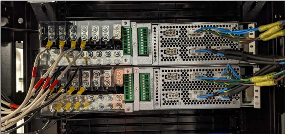
Figure 5: Wired Power Chassis
