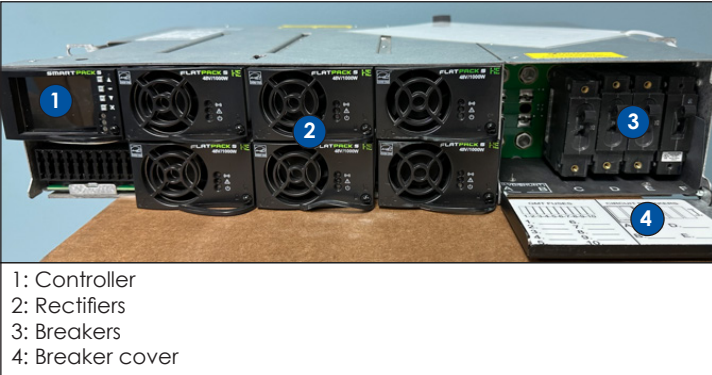
Figure 8: Eltek Shelf with Components
