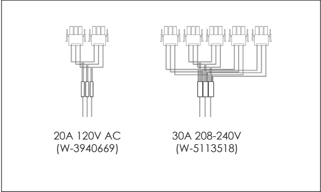
Figure 1: AC Connector Harness Options
