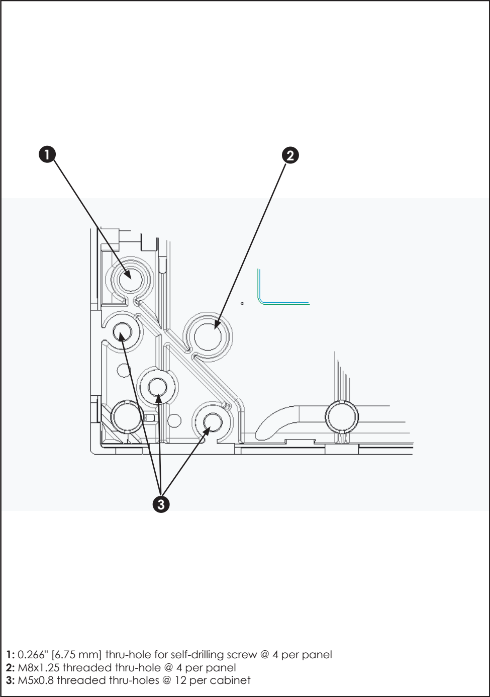
Figure 2: Detail A
