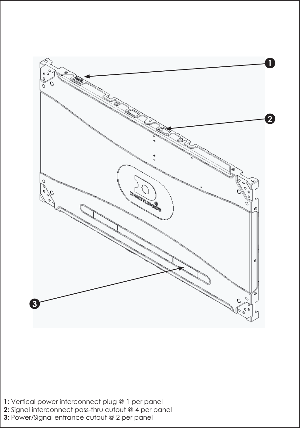
Figure 3: Rear View
