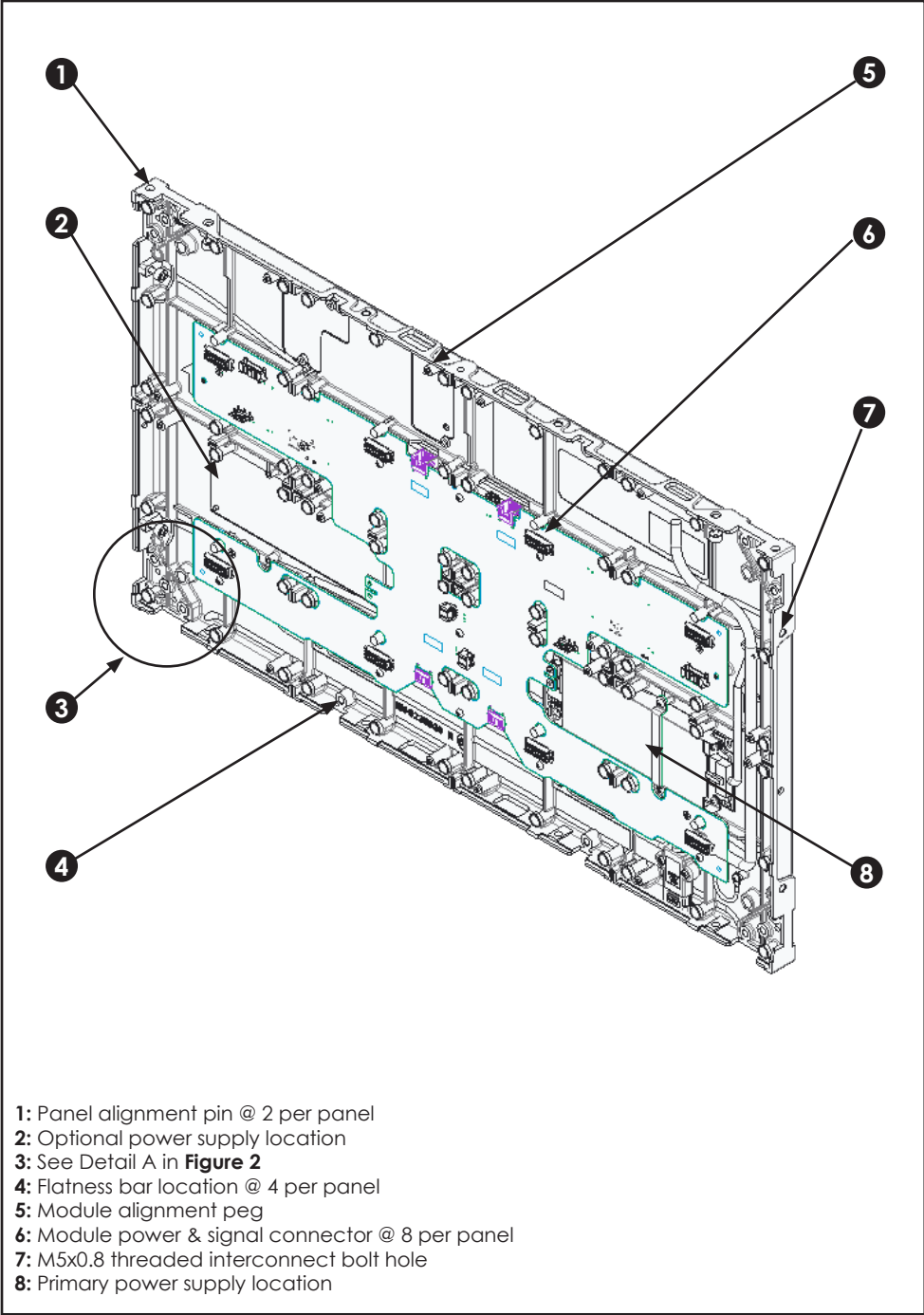
Figure 1: Front View
