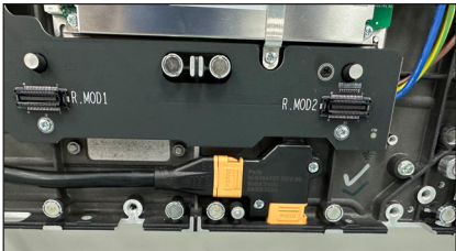
Figure 20: Install Power Input Cable
