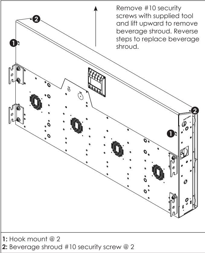
Figure 2: Beverage Shroud Removal
