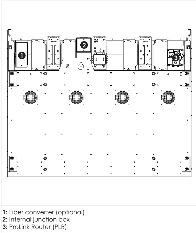
Figure 7: Component Locations (Rear View with Beverage Shroud Removed)
