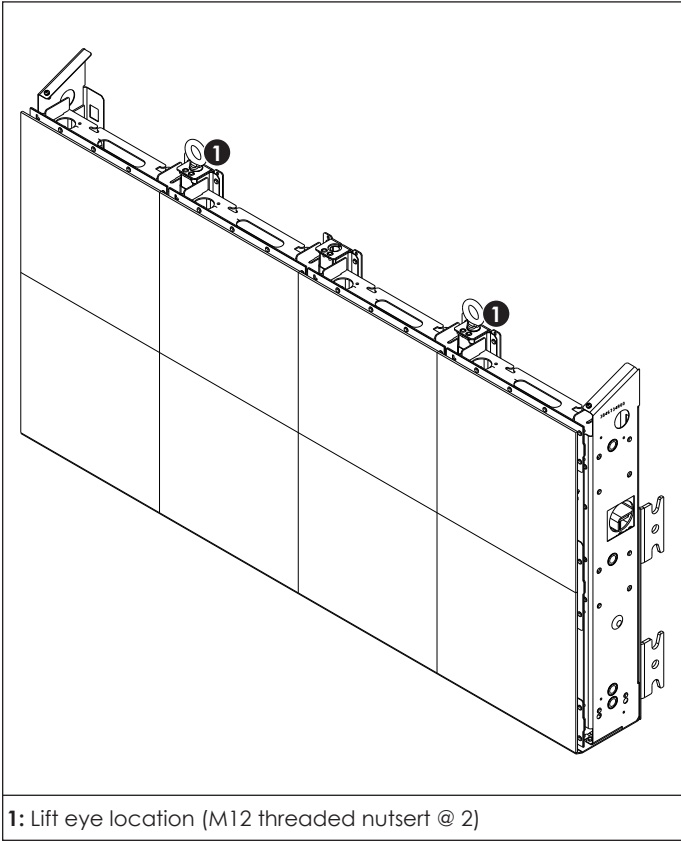
Figure 1: Display Front (Beverage Shroud Removed)
