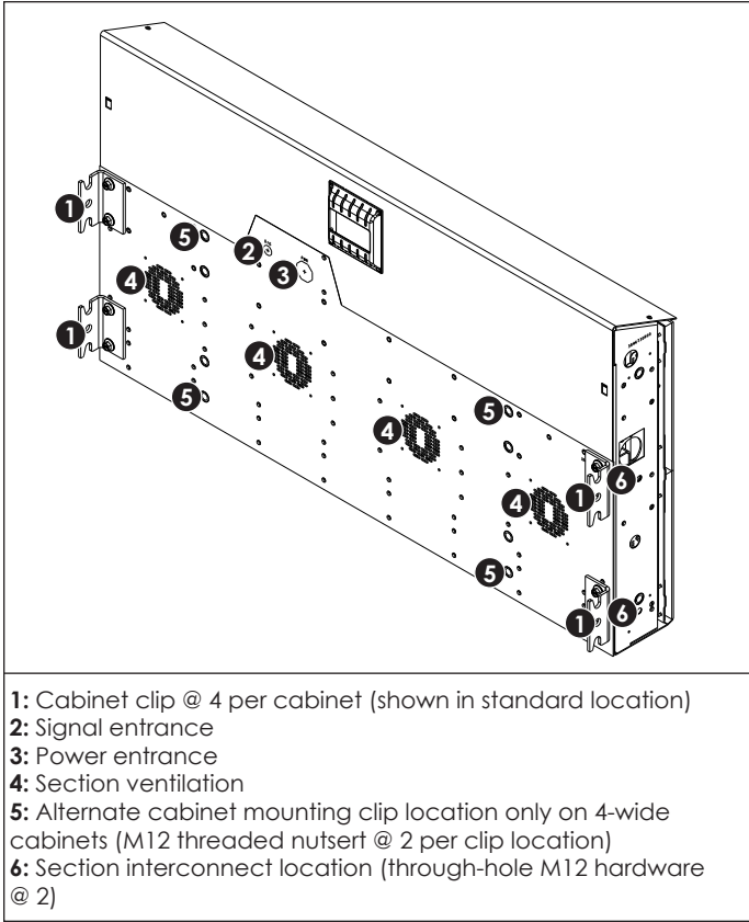
Figure 3: Display Rear without External Support Structure
