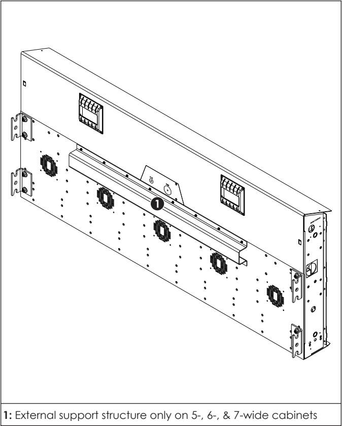
Figure 4: Display Rear with External Support Structure
