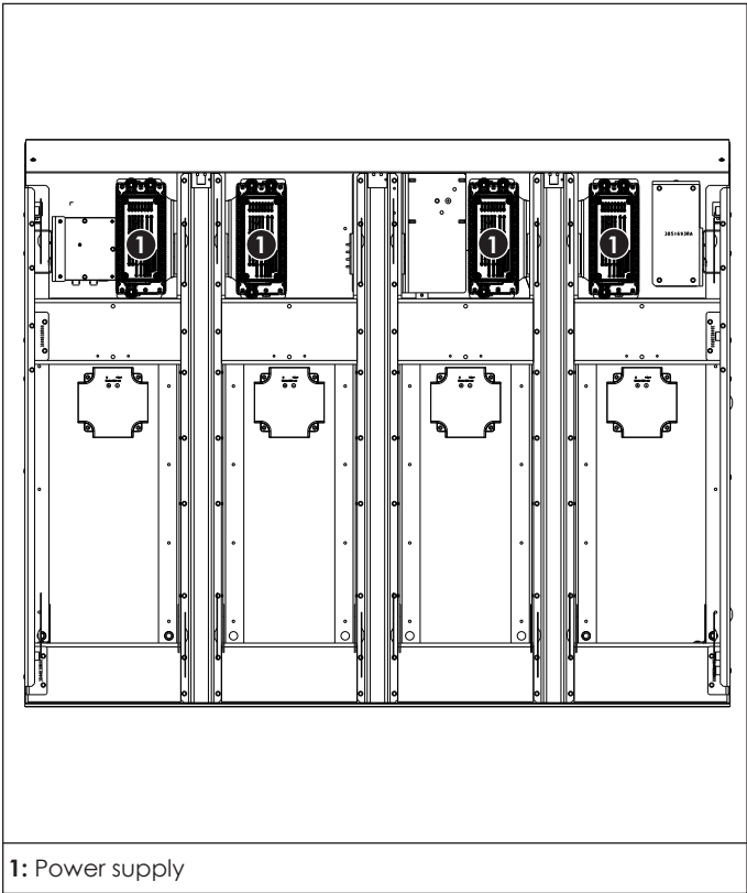
Figure 6: Component Locations (Front View with Module Column Removed)
