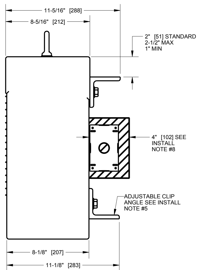
DETAILED RIGHT VIEW SCALE 1/5
