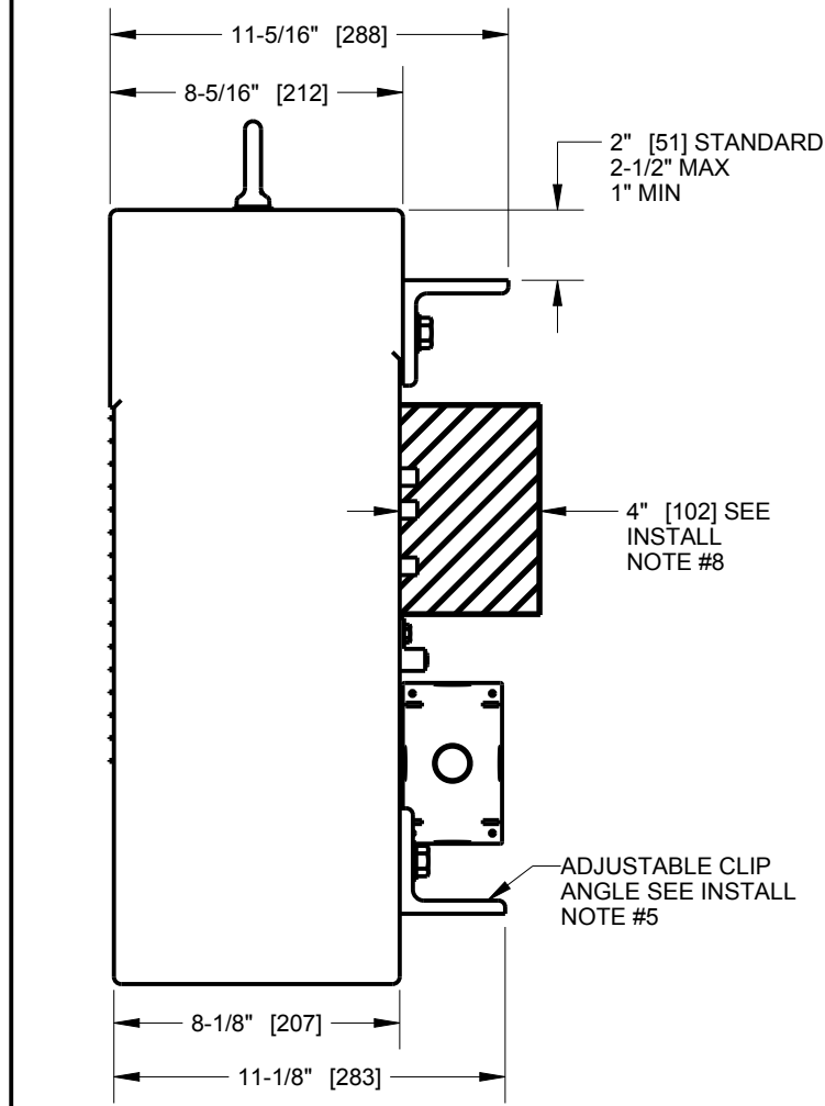
DETAILED RIGHT VIEW SCALE 1/6
