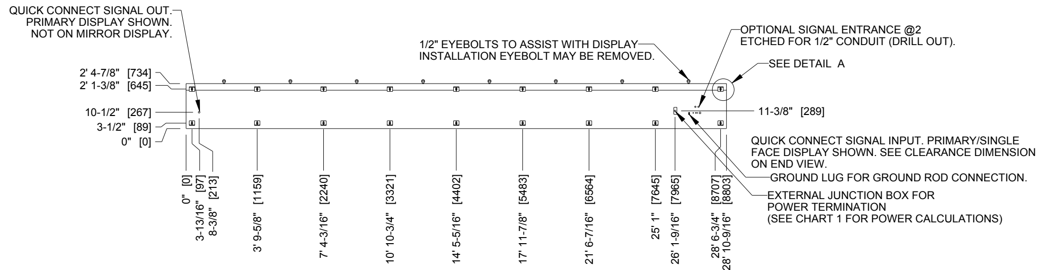
REAR VIEW
