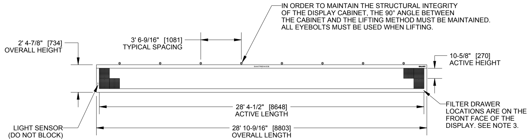
FRONT VIEW
