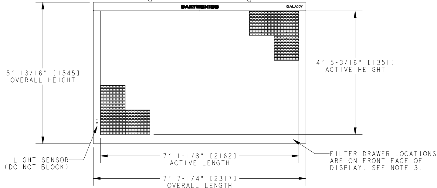
FRONT VIEW
