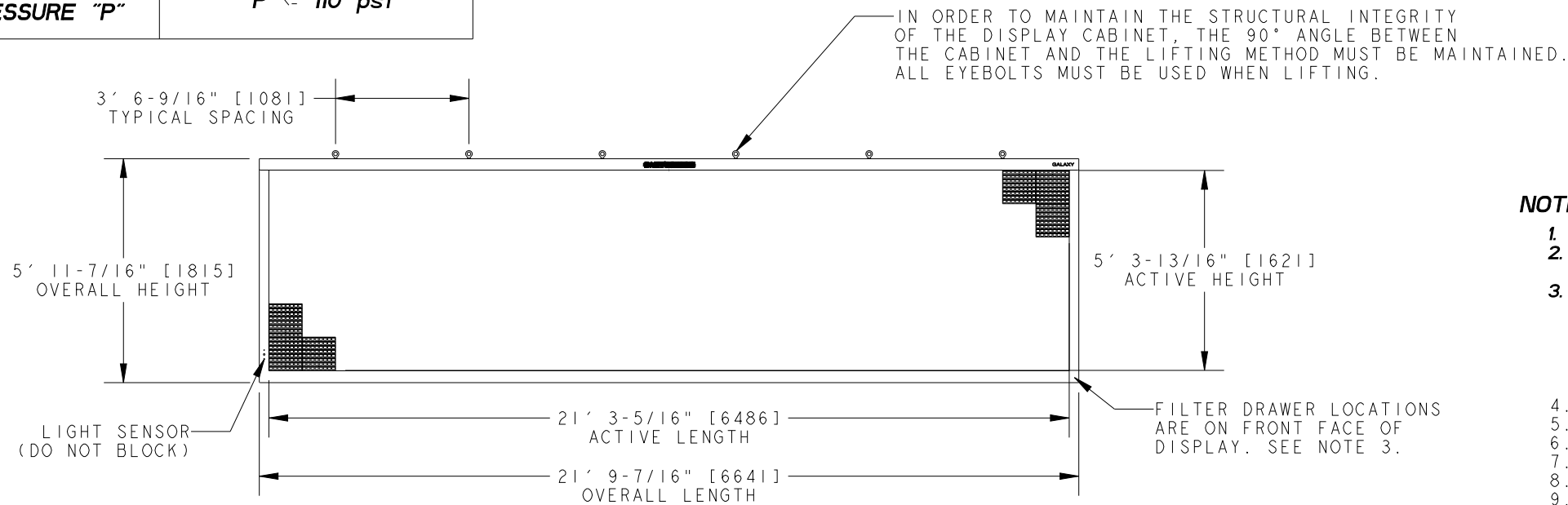
FRONT VIEW
