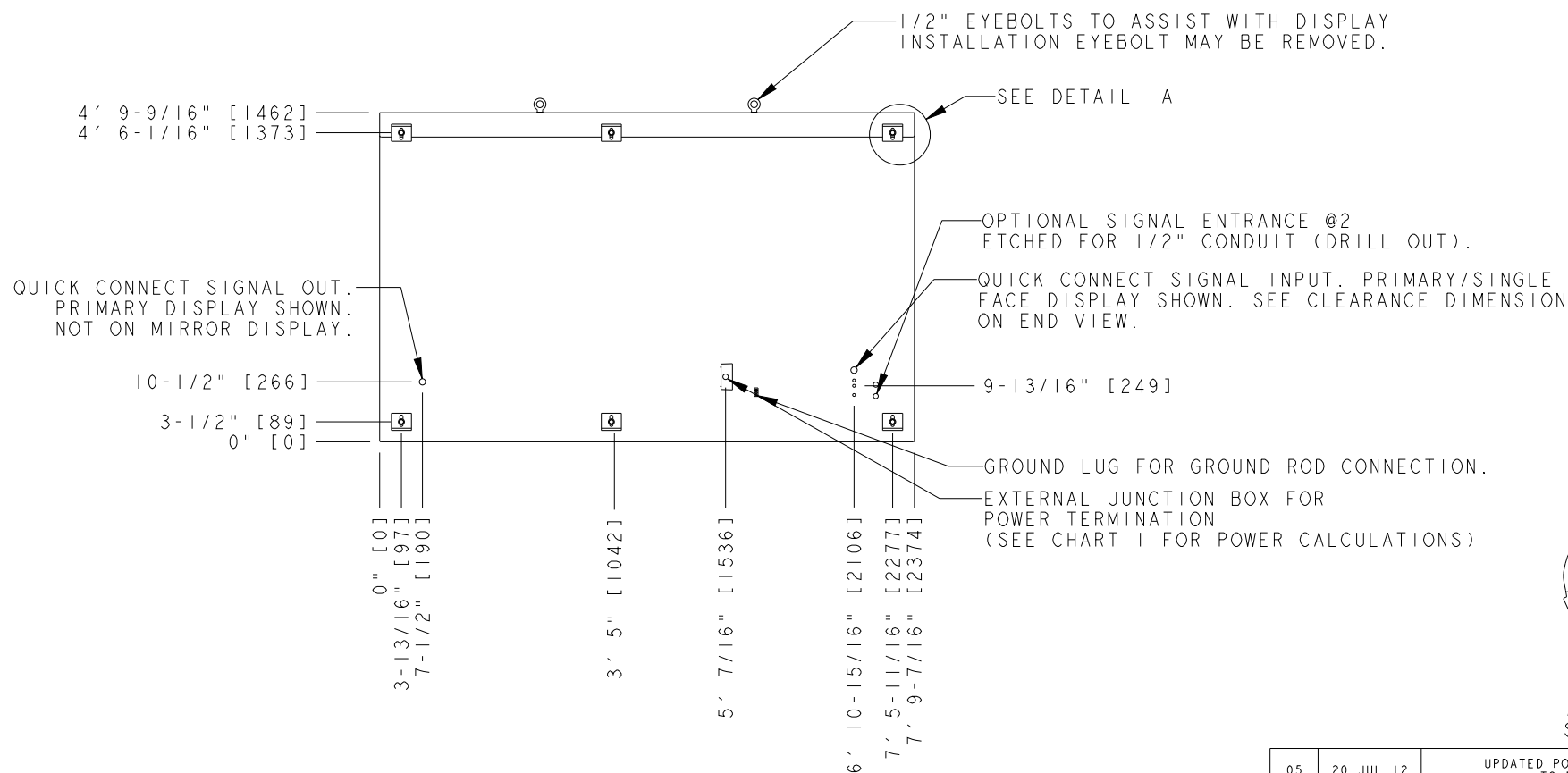
REAR VIEW
