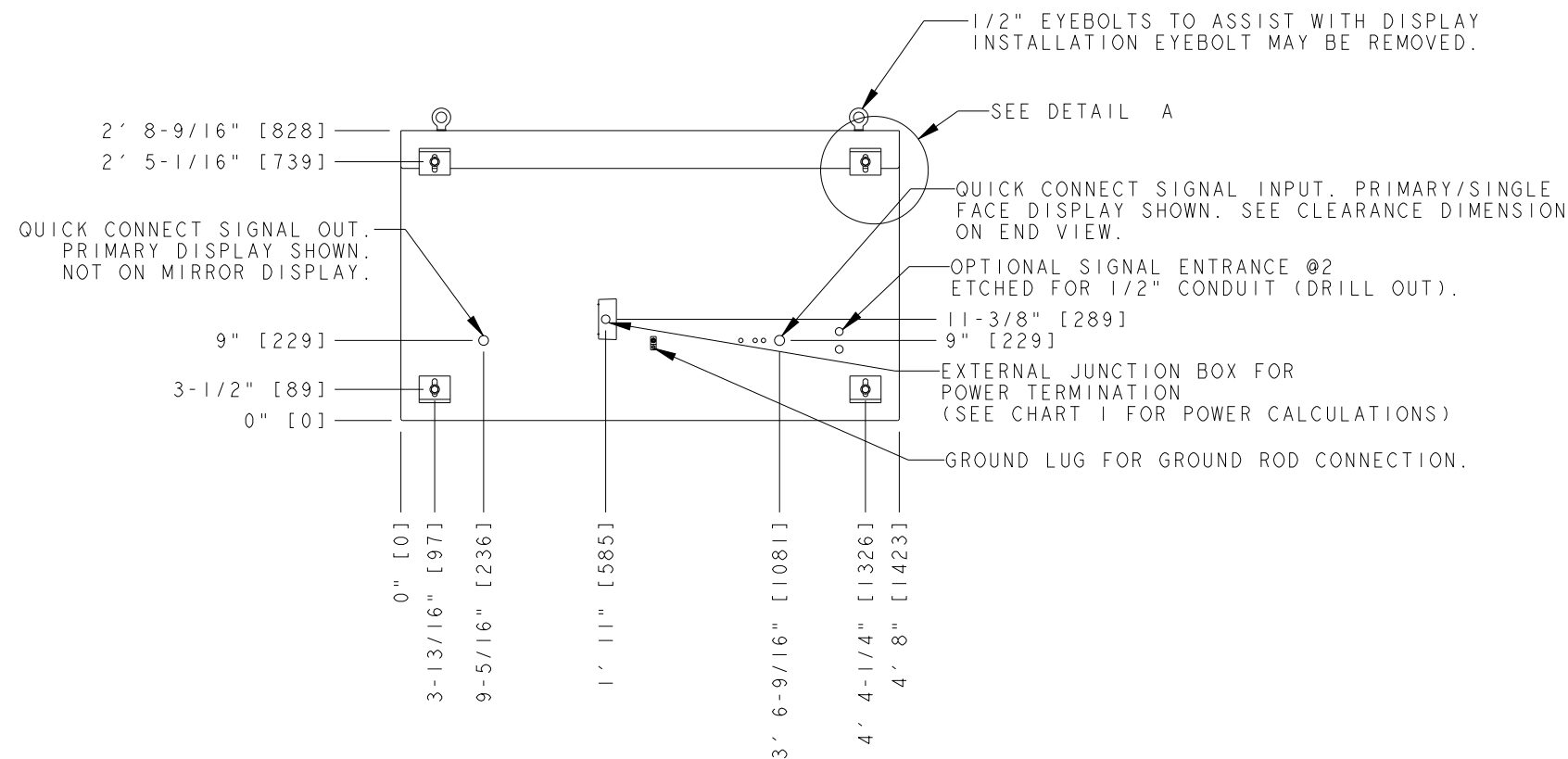
REAR VIEW
