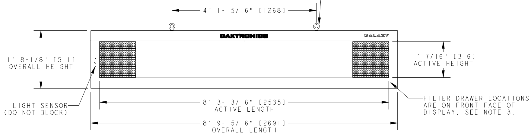
FRONT VIEW
