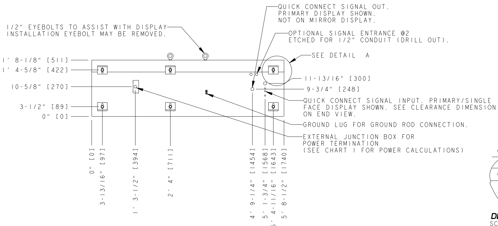
REAR VIEW
