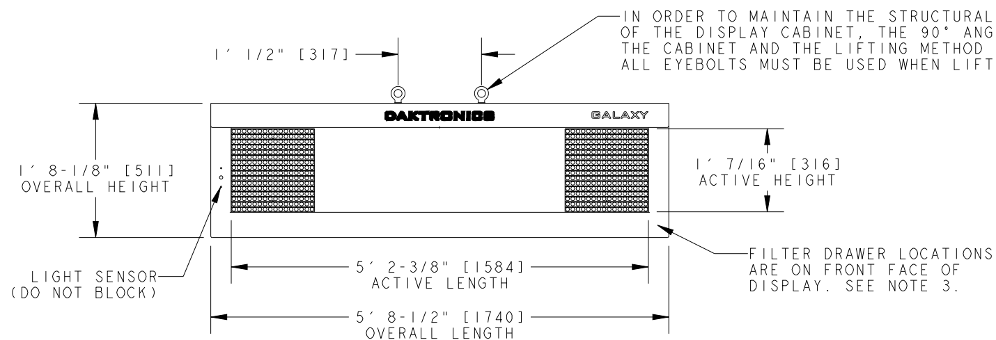
FRONT VIEW
