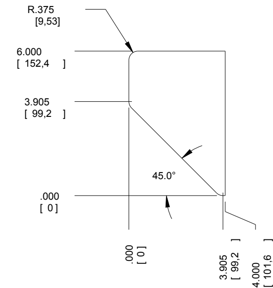
PART A MATERIAL: 1/2" [12,7] ASTM A36 STEEL
