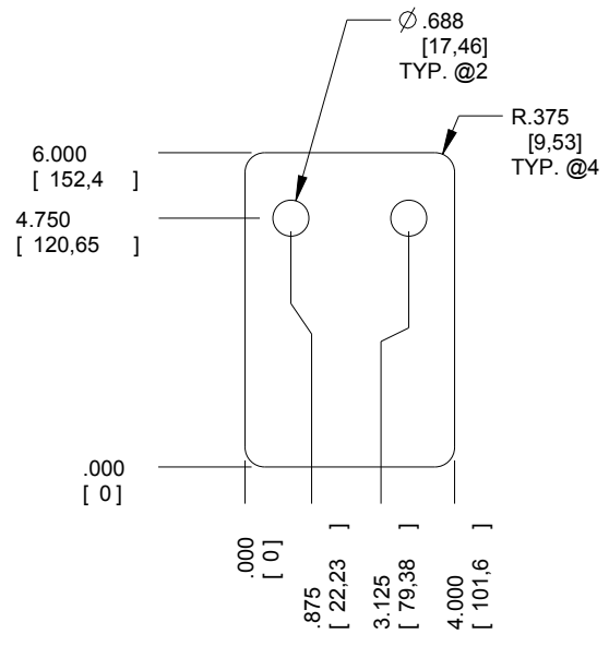
PART B MATERIAL: 1/2" [12,7] ASTM A36 STEEL
