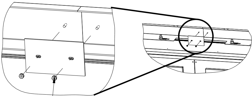
BORDER SPLICE ATTACHMENT
