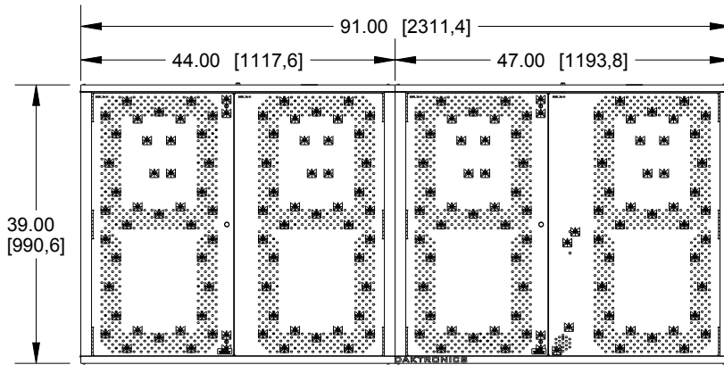
FRONT VIEW
