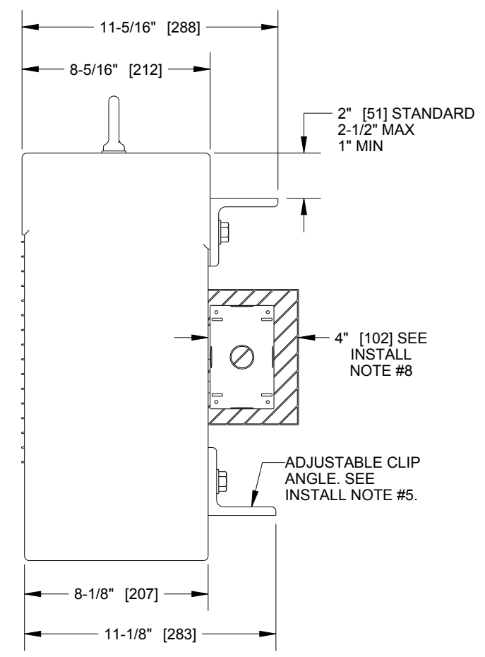
DETAILED RIGHT VIEW SCALE 67/400
