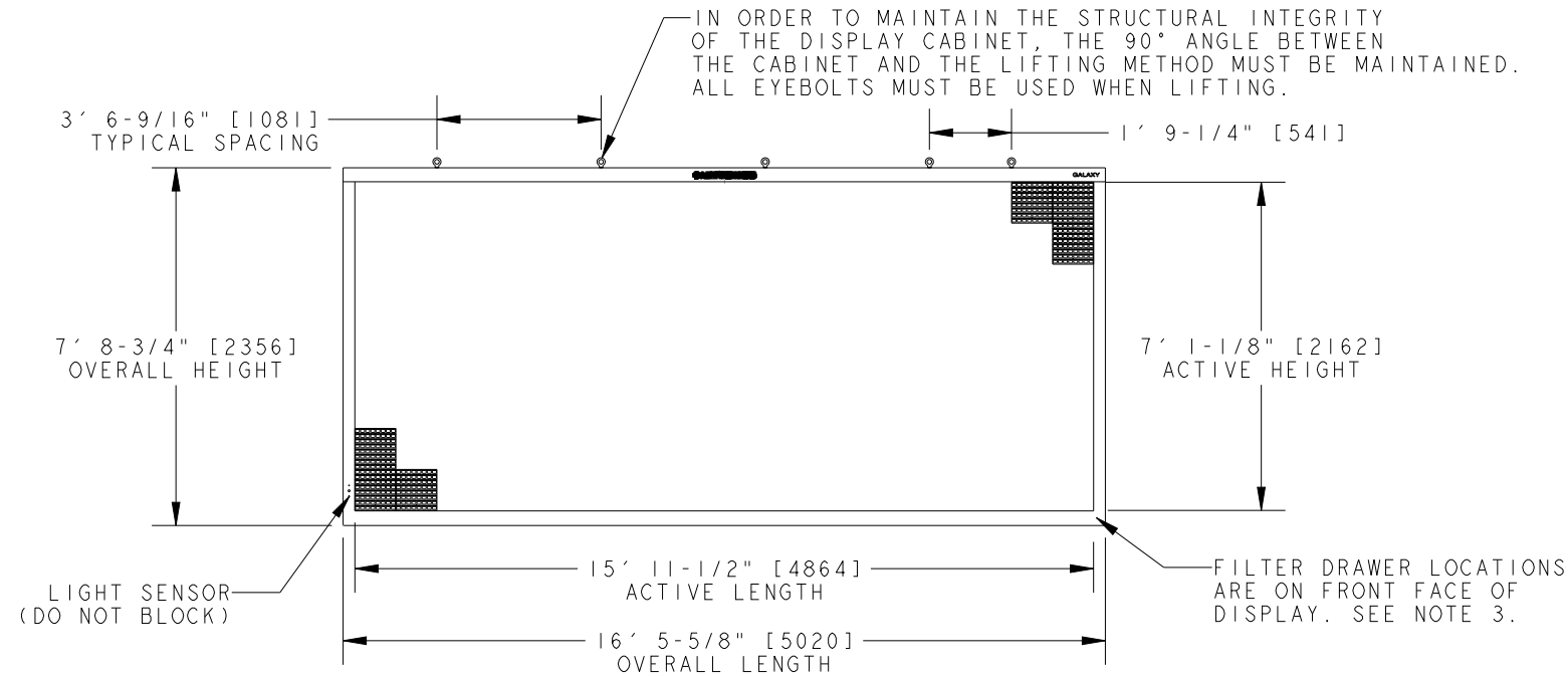
FRONT VIEW
