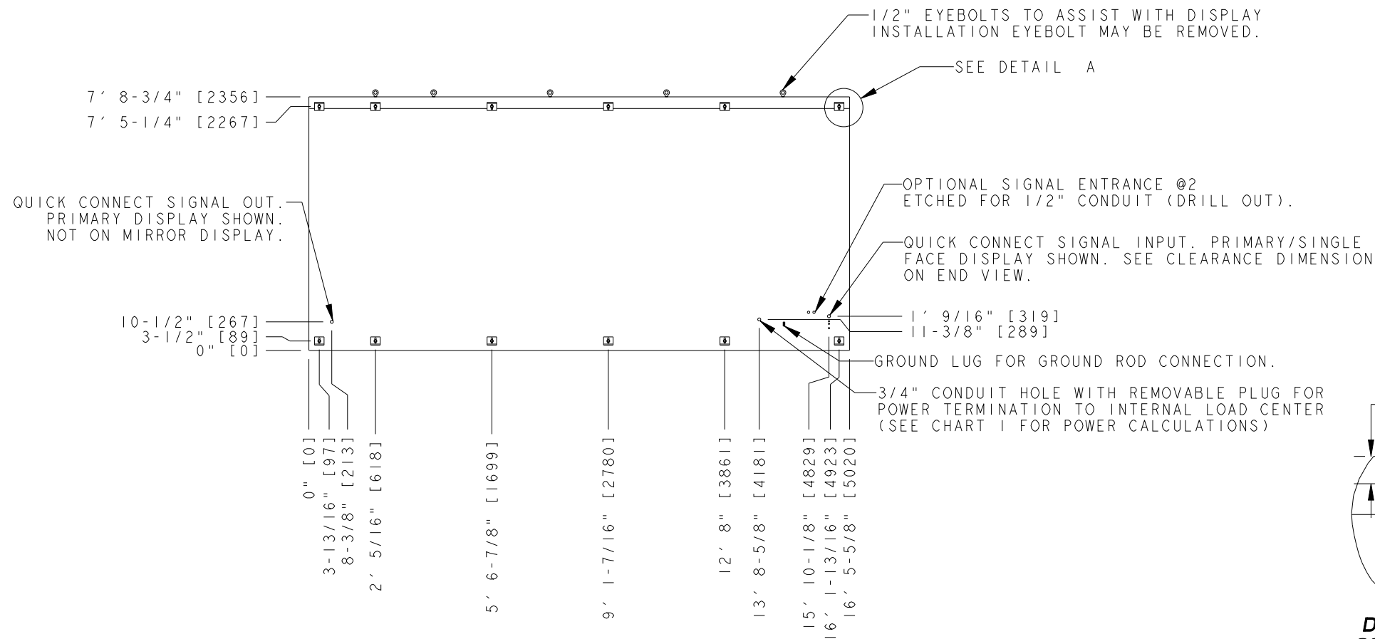
REAR VIEW
