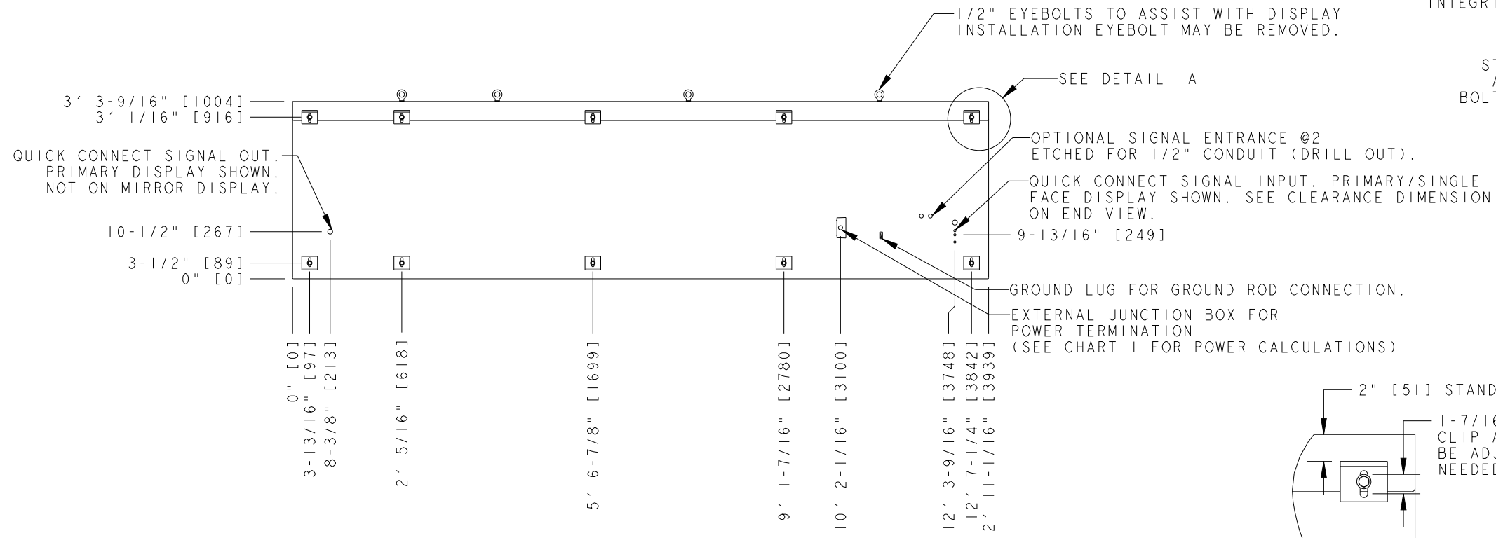
FRONT VIEW
