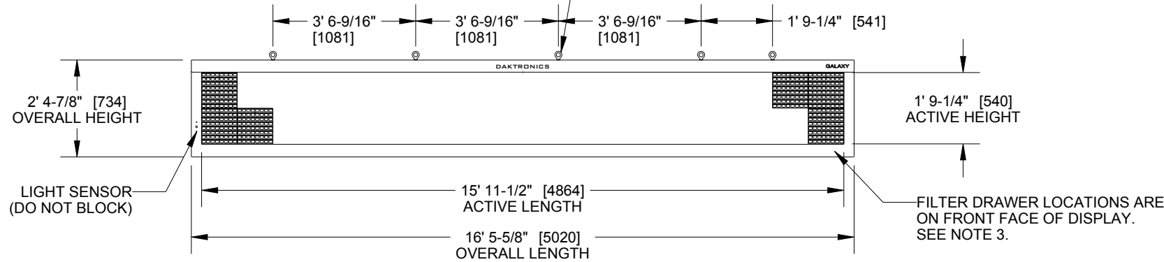
FRONT VIEW
