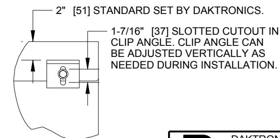
DETAIL A SCALE 1/10
