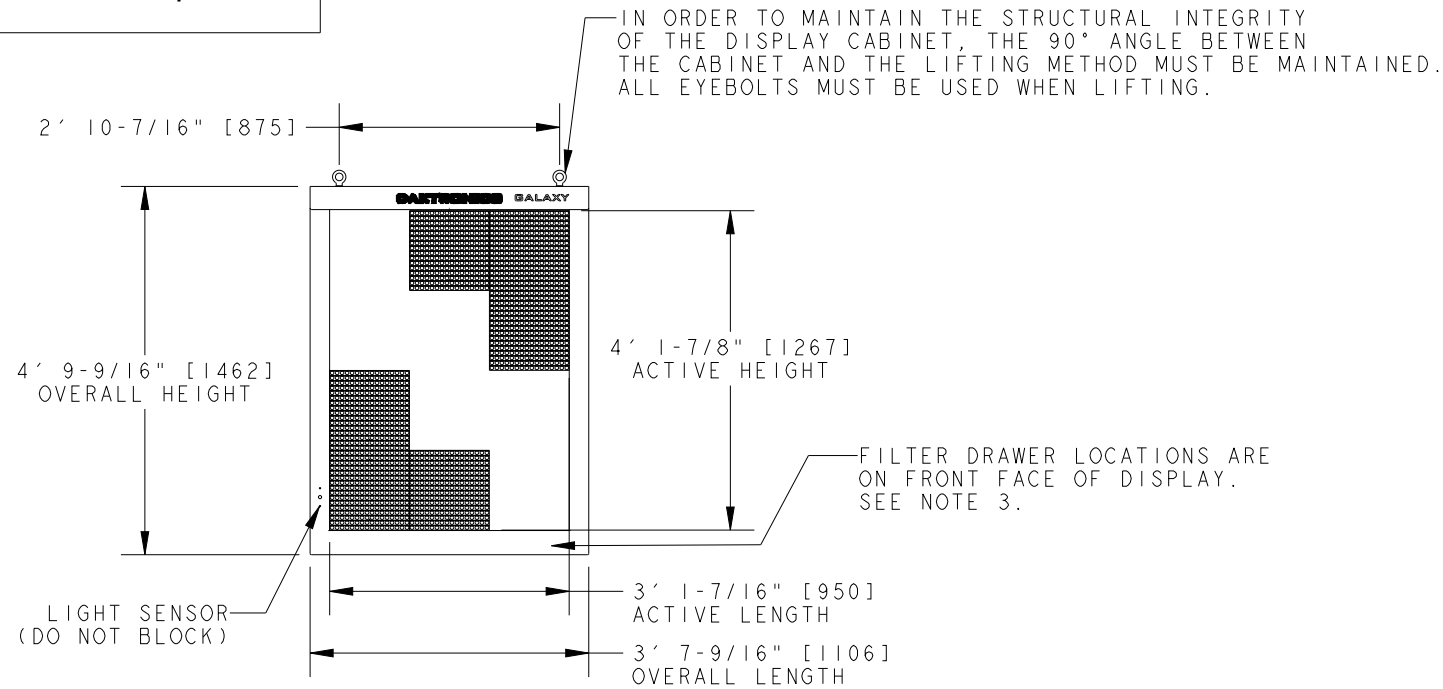
FRONT VIEW
