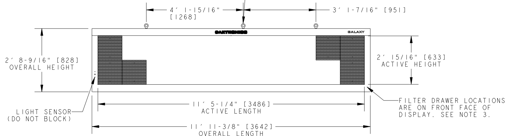
FRONT VIEW
