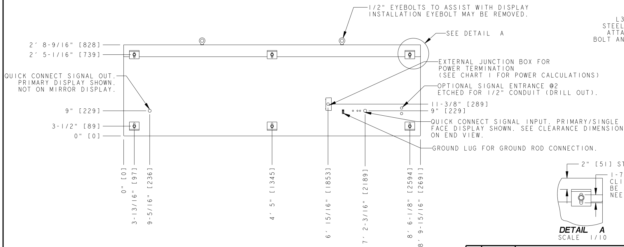
REAR VIEW
