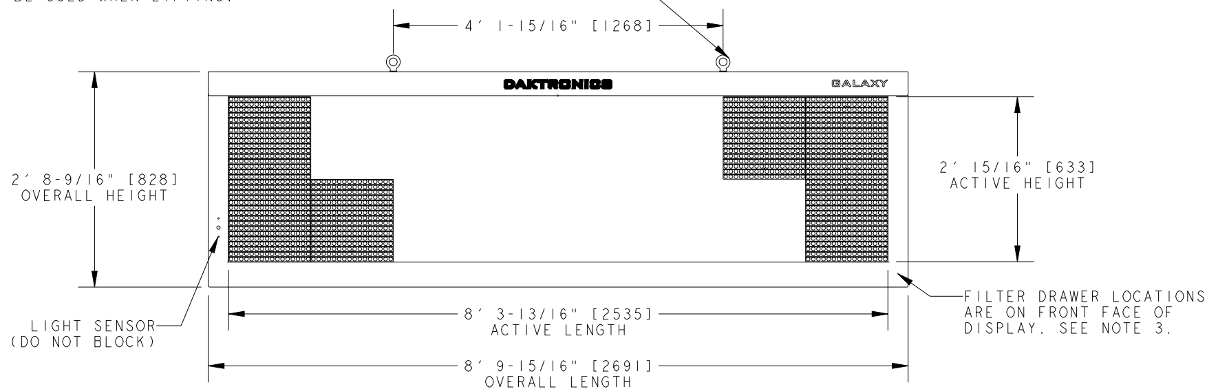
FRONT VIEW
